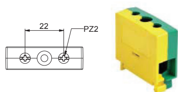
KC 1X16
